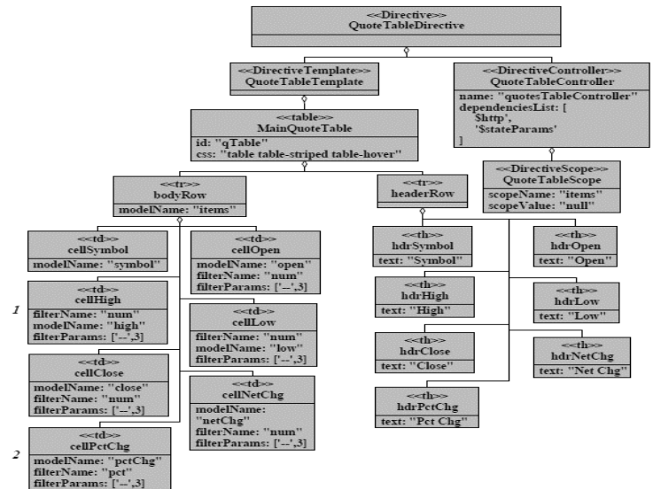
Fig. 5. Directive part of design model of case study.
