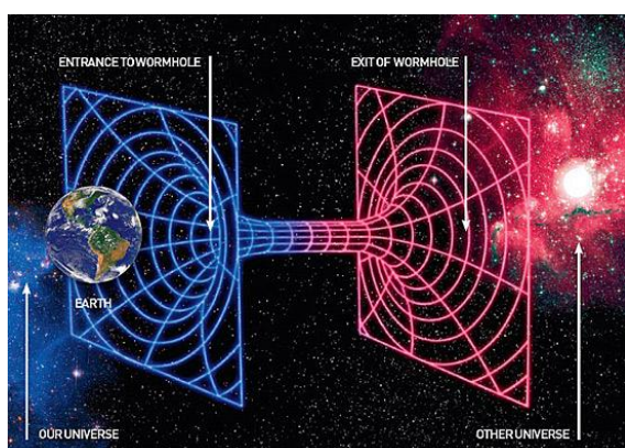
Fig 7: Wormhole
