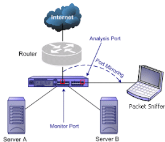
Fig 2. Packet sniffing in switched environment
