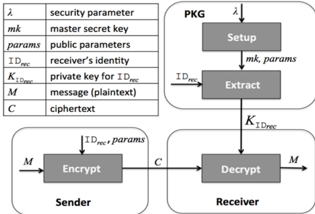
FIGURE 1. OVERVIEW OF IDENTITY-BASED ENCRYPTION
